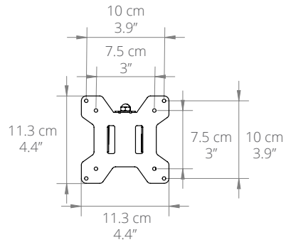
DETACHABLE MONITOR PLATE
